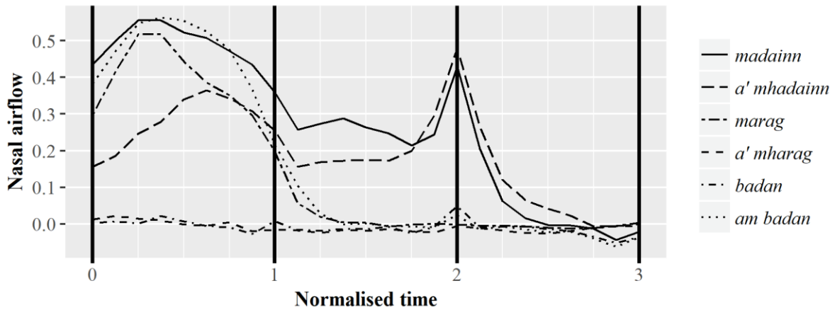
Fig. 1: Dynamic nasal airflow profiles for the underlined portions of madainn [mātəp̪] 'morning', a' mhadainn [ə vātəp̪] 'the morning', marag [marak] 'pudding', a' mharag [ə varak] 'the pudding', badan [patan] 'thicket' and am badan [ə matan] (< /əm patan/) 'the thicket'. The x-axis represents normalised time, where 0-1 is the duration of the initial consonant, 1-2 is the duration of the vowel, and 2-3 is the duration of the following consonant.
