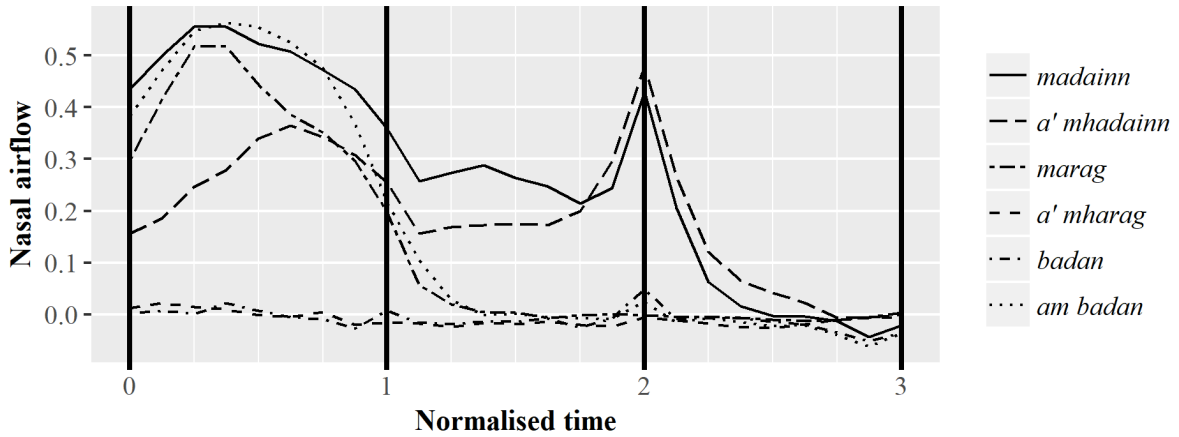
Fig. 1: Dynamic nasal airflow profiles for the underlined portions of madainn [mātəp̪i] 'morning', a' mhadainn [ə vātəp̪i] 'the morning', marag [marak] 'pudding', a' mharag [ə varak] 'the pudding', badan [patan] 'thicket' and am badan [ə matan] (< /əm patan/) 'the thicket'. The x-axis represents normalised time, where 0-1 is the duration of the initial consonant, 1-2 is the duration of the vowel, and 2-3 is the duration of the following consonant.
